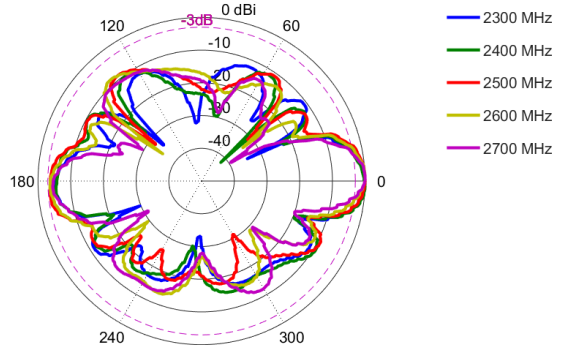
Elevation: 2300 - 2700 MHz
