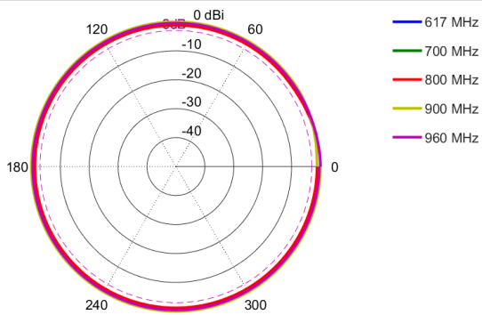
Azimuth: 617 - 960 MHz
