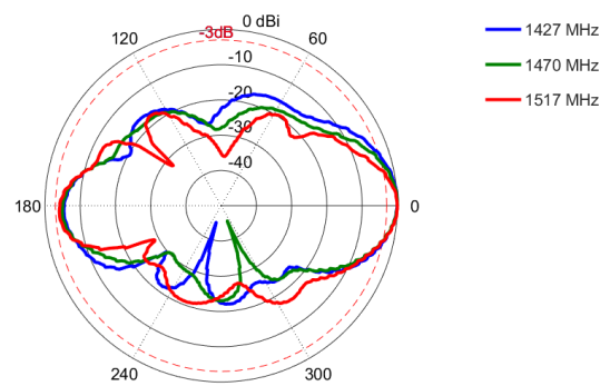
Elevation: 1427 - 1517 MHz
