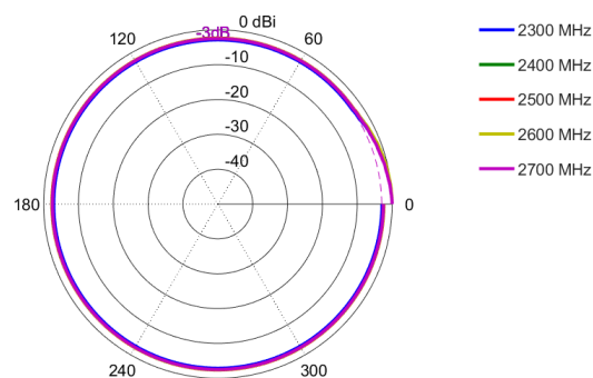
Azimuth: 2300 - 2700 MHz
