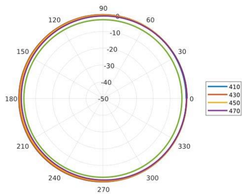
Azimuth: 410 – 470 MHz
