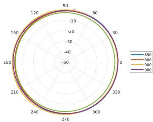
Azimuth: 690 – 960 MHz
