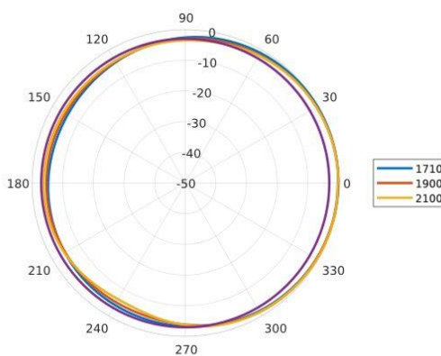
Azimuth: 1710 – 2100 MHz
