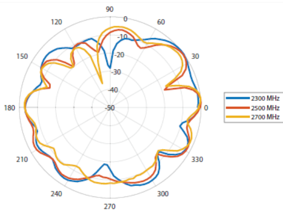
Elevation: 2300 – 2700 MHz
