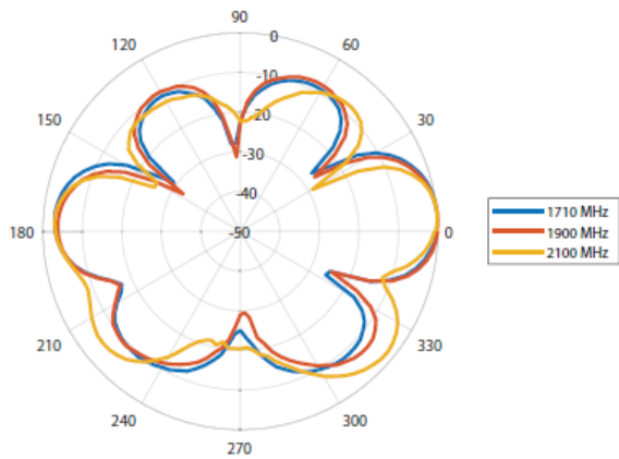
Elevation: 1710 – 2170 MHz
