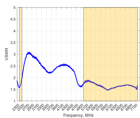
VSWR: Wi-Fi Antenna
