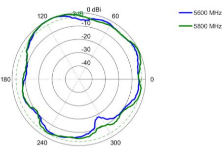
Elevation 2: 5600 – 5800 MHz
