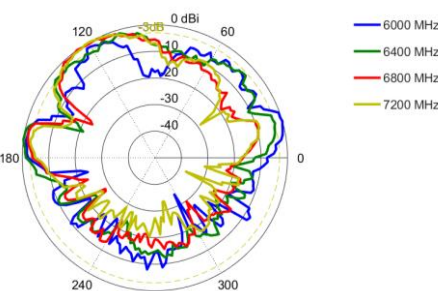
Elevation 1: 6000 – 7200 MHz
