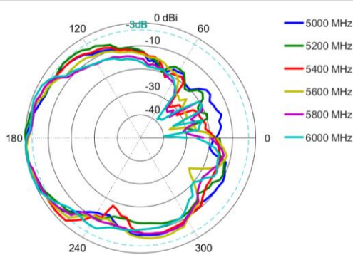
Azimuth: 5000 – 6000MHz
