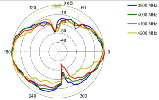
Elevation: 3900 – 4200 MHz
