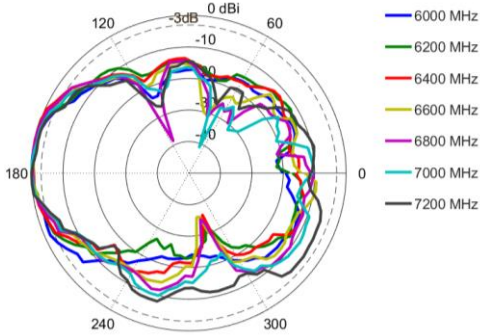
Azimuth: 6000 – 7200 MHz
