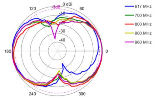
Elevation: 617 – 960 MHz
