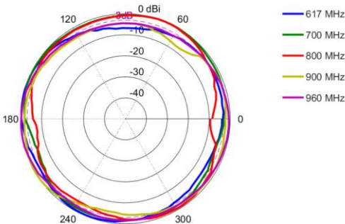
Azimuth: 617 – 960 MHz
