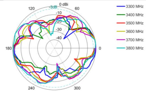
Elevation: 3300 – 3800 MHz
