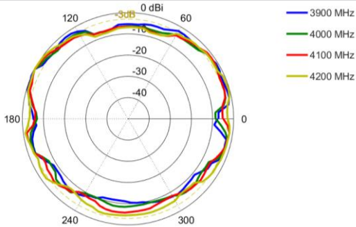
Azimuth: 3900 – 4200 MHz
