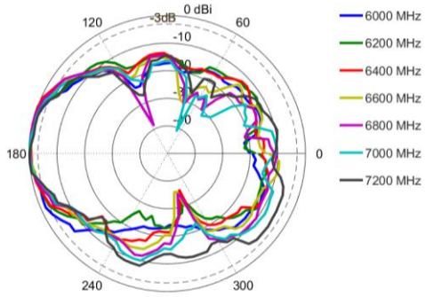
Elevation: 6000 – 7200 MHz
