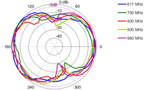
Elevation: 617 – 960 MHz
