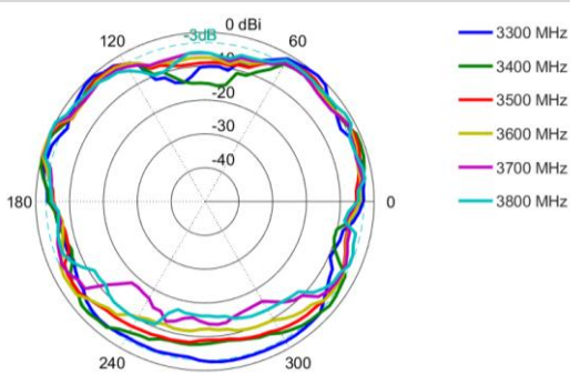
Azimuth: 3300 – 3800 MHz
