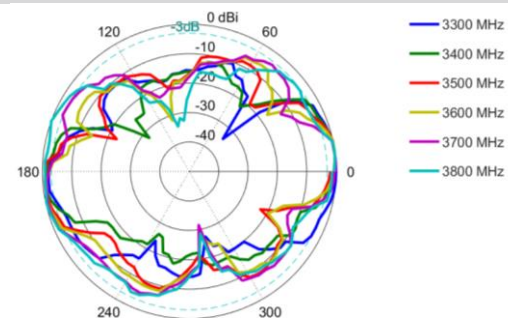
Elevation: 3300 – 3800 MHz
