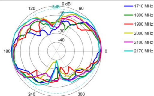
Elevation: 1710 – 2170 MHz
