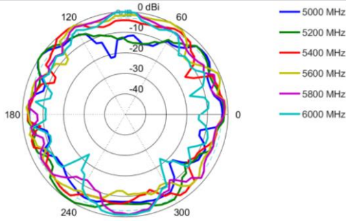
Azimuth: 5000 – 6000 MHz
