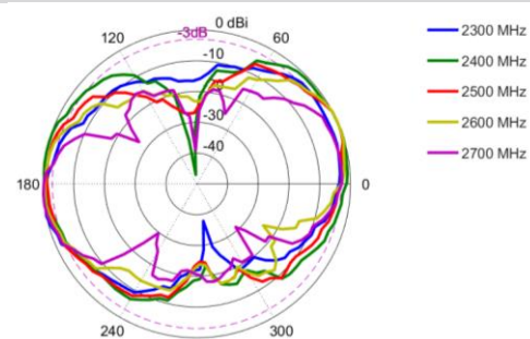
Elevation: 2300 – 2700 MHz
