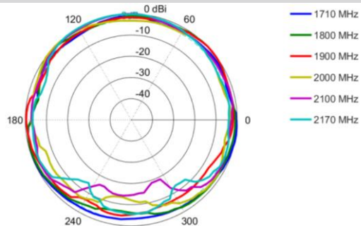
Azimuth: 1710 – 2170 MHz
