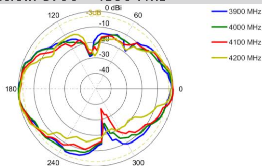
Elevation: 3900 – 4200 MHz
