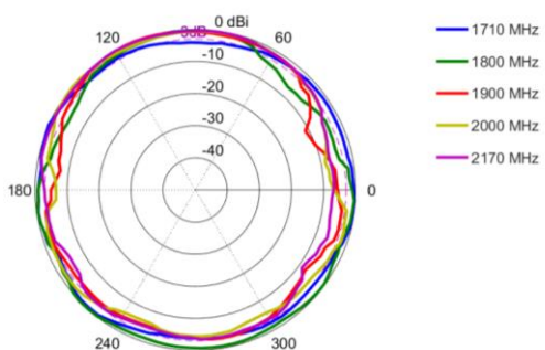
Azimuth: 1710 – 2170 MHz
