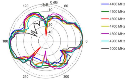
Elevation: 4400 – 5000 MHz
