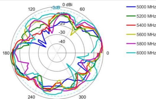
Elevation: 5000 – 6000 MHz
