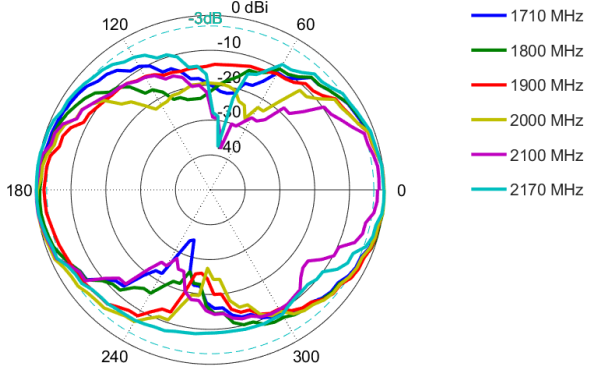
Elevation: 1710 – 2170MHz
