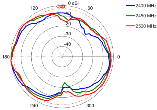
Elevation: 2400 – 2500MHz
