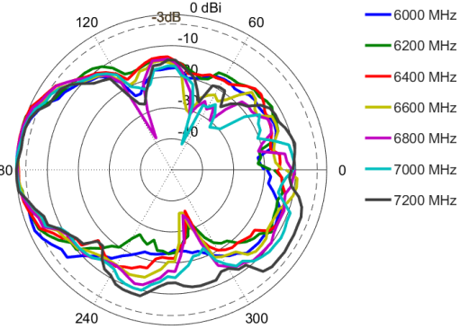
Elevation: 6000 – 7200 MHz
