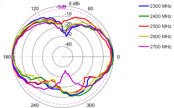
Elevation: 2300 – 2700MHz
