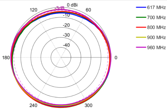
Azimuth: 617 – 960 MHz
