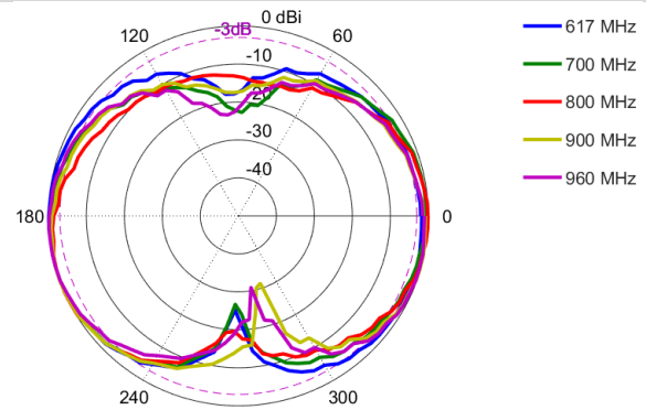
Elevation: 617 – 960 MHz
