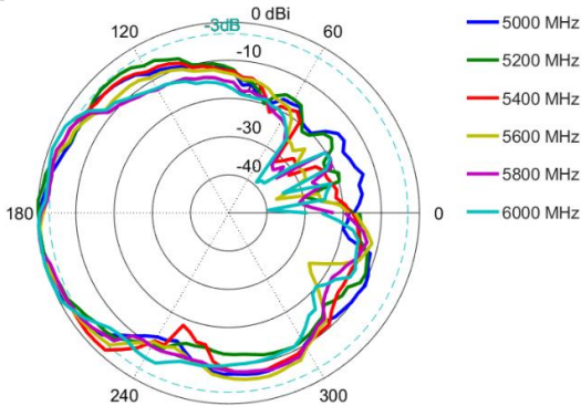
Azimuth: 5000 – 6000MHz
