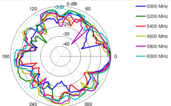
Elevation: 5000 – 6000 MHz
