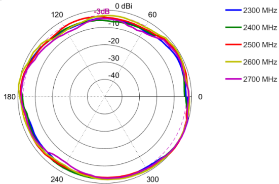
Azimuth: 2300 – 2700 MHz
