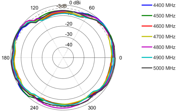
Azimuth: 4400 – 5000 MHz
