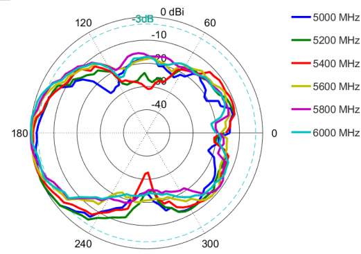
Elevation: 5000 – 6000MHz
