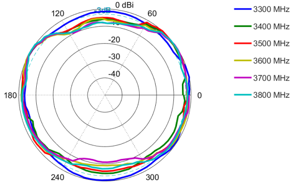
Azimuth: 3300 – 3800 MHz
