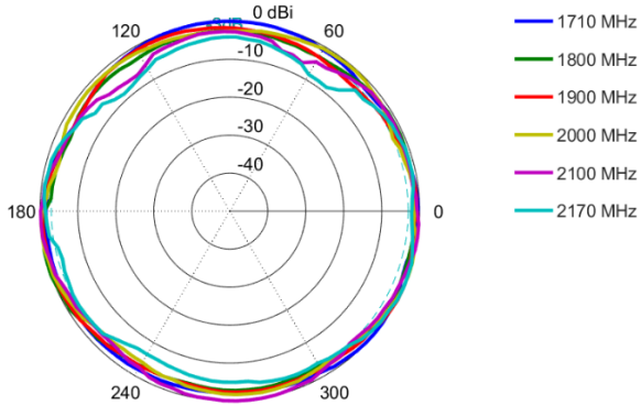
Azimuth: 1710 – 2170 MHz
