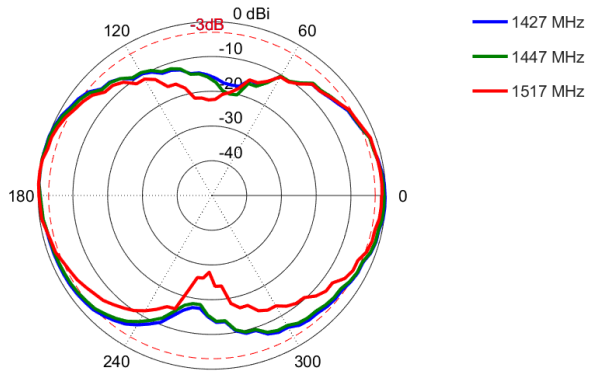
Elevation: 1427 – 1517 MHz
