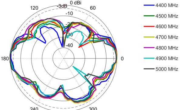
Elevation: 4400 – 5000 MHz
