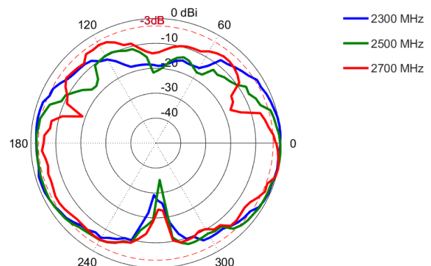
Elevation: 2300 – 2700 MHz
