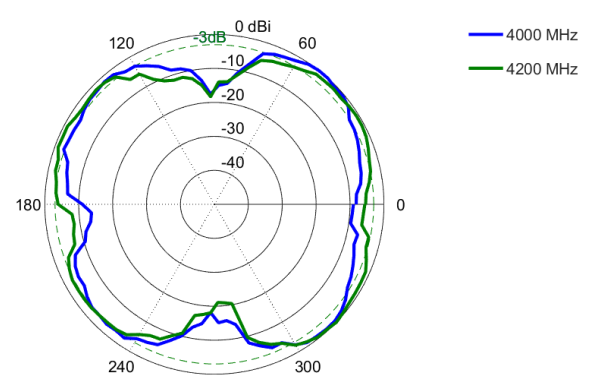
Elevation: 4000 – 4200 MHz
