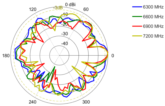
Elevation: 6300 – 7200 MHz
