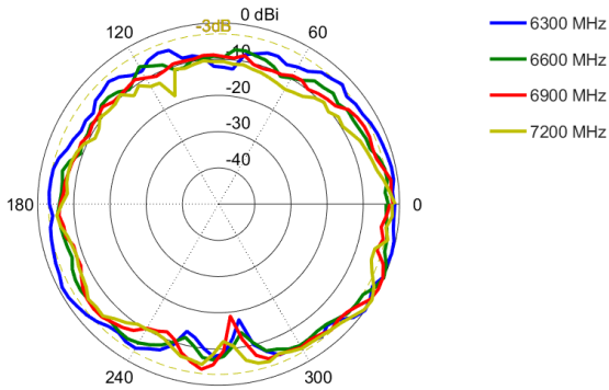
Azimuth: 6300 – 7200 MHz
