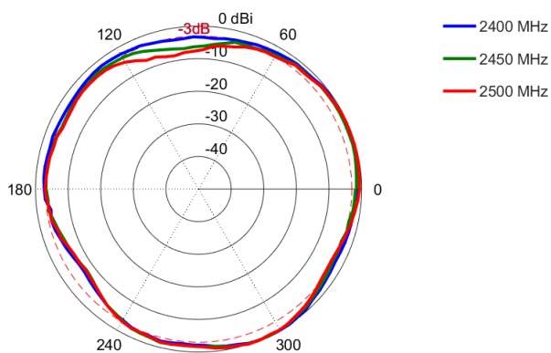
Azimuth: 2400 – 2500 MHz
