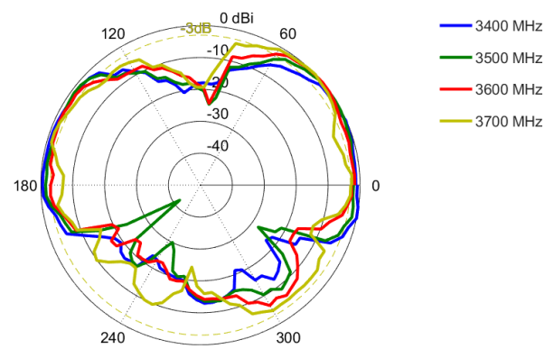
Elevation: 3400 – 3700 MHz
