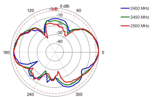
Elevation: 2400 – 2500 MHz
