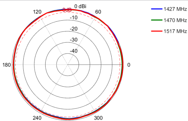
Azimuth: 1427 – 1517 MHz
