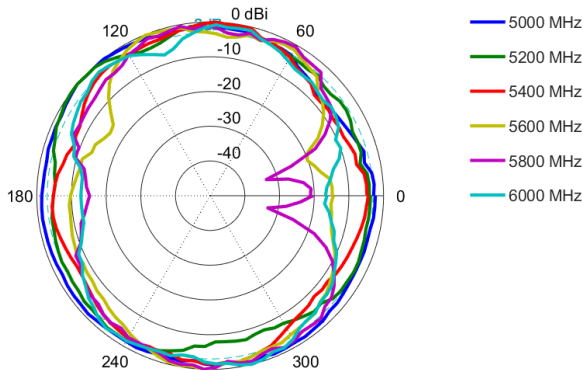
Azimuth: 5000 – 6000 MHz
