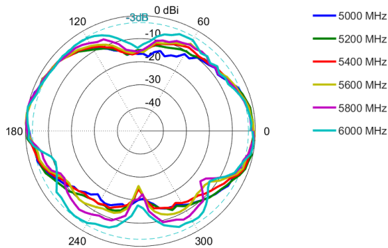
Elevation: 5000 – 6000 MHz
