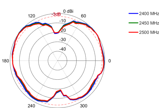
Elevation: 2400 – 2500 MHz
