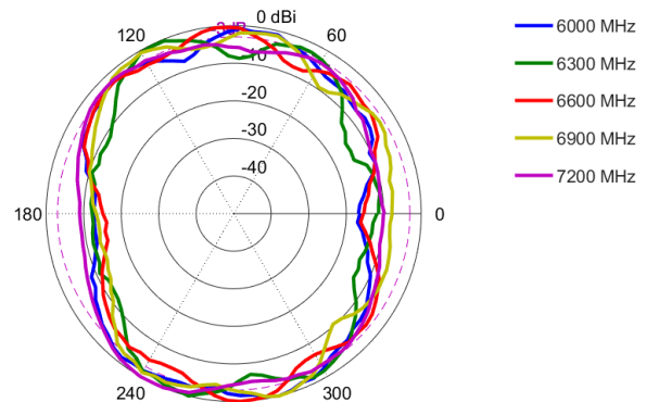
Azimuth: 6000 – 7200 MHz
