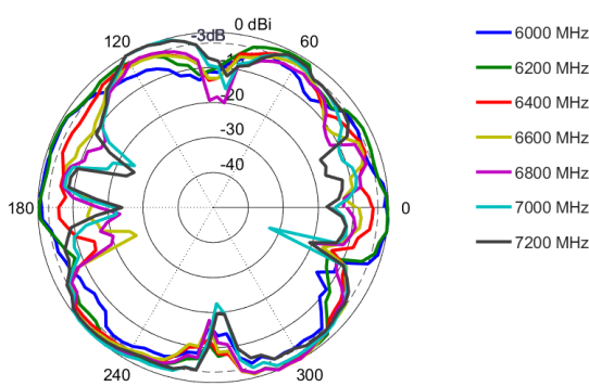
Elevation: 6000 – 7200 MHz
