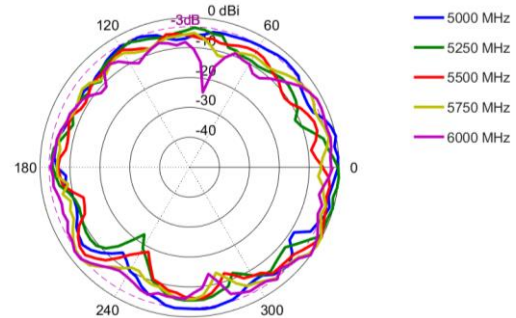
Azimuth: 5000 – 6000 MHz
