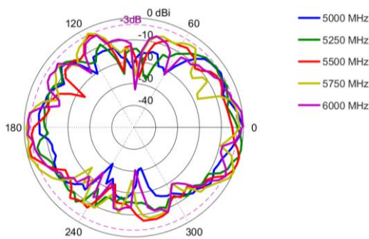
Elevation: 5000 - 6000 MHz
