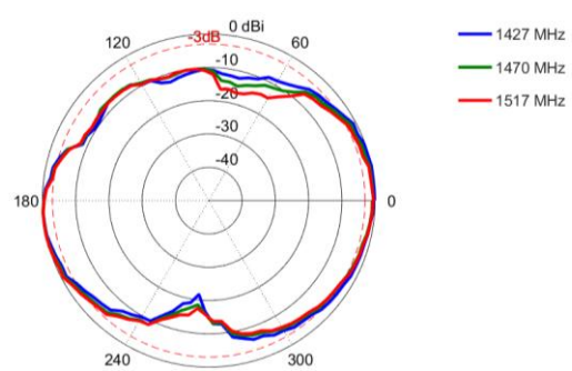
Elevation: 1427 – 1517 MHz
