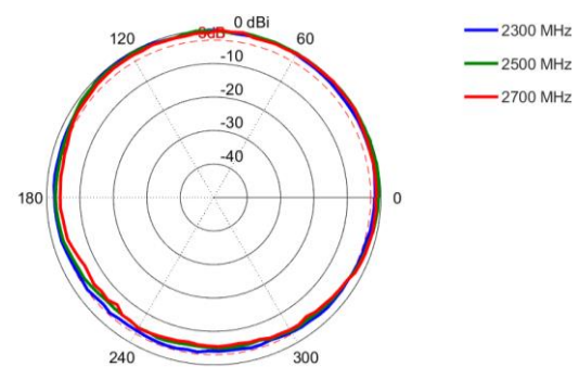
Azimuth: 2300 – 2700 MHz
