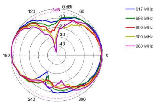
Elevation: 617 – 960 MHz
