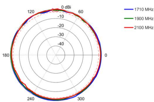
Azimuth: 1710 – 2100 MHz
