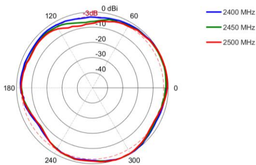
Azimuth: 2400 – 2500 MHz
