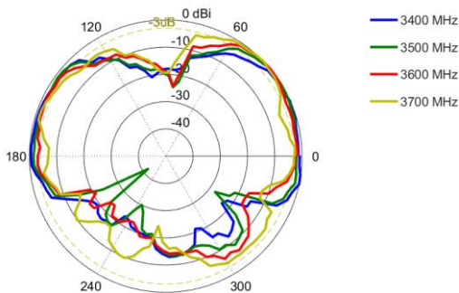
Elevation: 3400 – 3700 MHz
