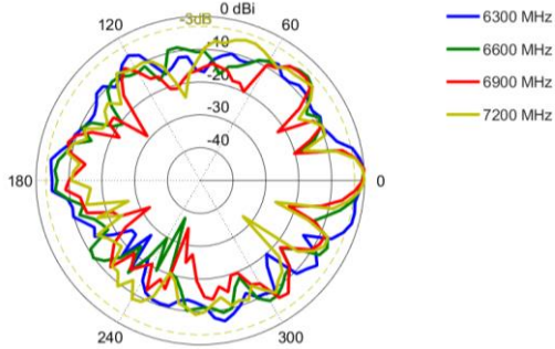
Elevation: 6300 - 7200 MHz
