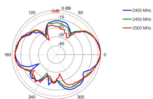
Elevation: 2400 – 2500 MHz
