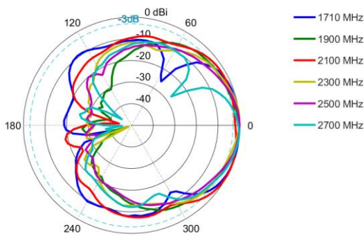
Elevation: 1710 – 2700 MHz
