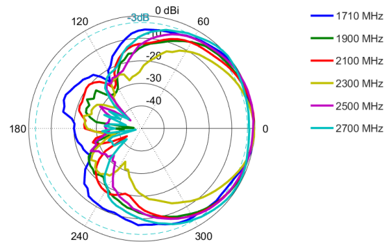
Azimuth: 1710 – 2700 MHz
