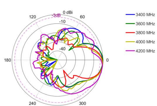
Elevation: 3400 – 4200 MHz
