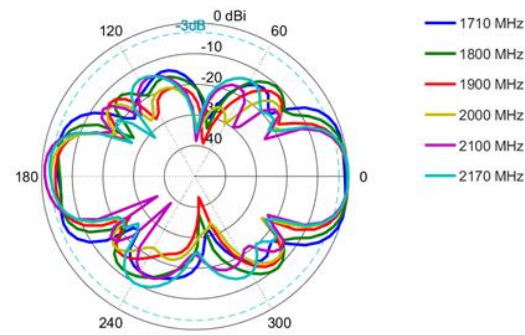
Elevation: 1710 – 2170 MHz
