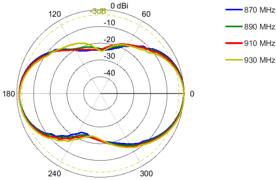
Elevation: 868 - 930 MHz
