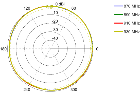
Azimuth: 868 - 930 MHz
