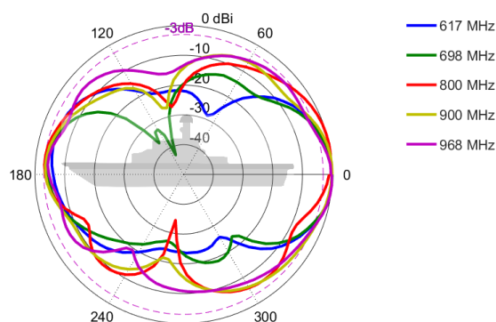
Elevation: 617 – 968 MHz
