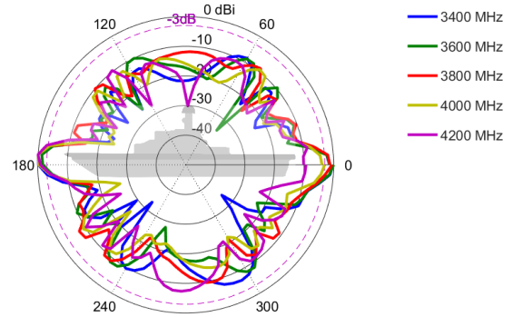
Elevation: 3400 – 4200 MHz
