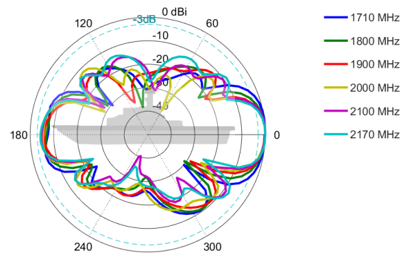
Elevation: 1710 – 2170 MHz
