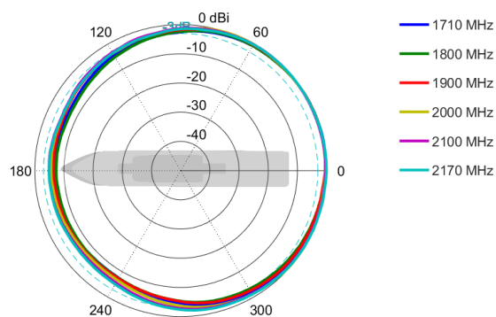
Azimuth: 1710 – 2170 MHz
