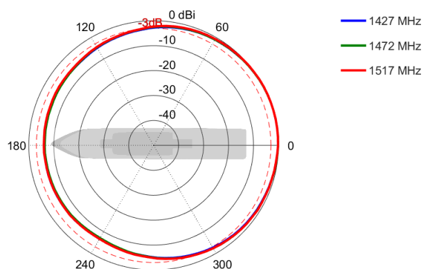
Azimuth: 1427 – 1517 MHz
