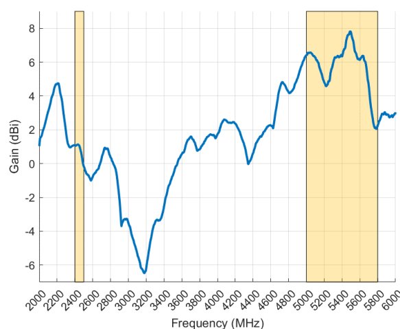
Gain: Wi-Fi Antenna
