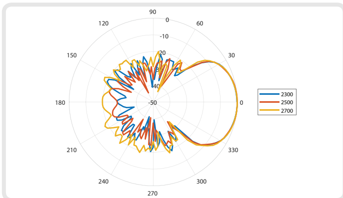
Azimuth: 2300 - 2700 MHz
