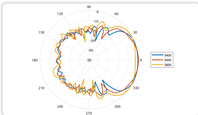
Azimuth: 3400 - 3800 MHz
