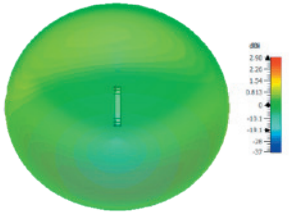
3D Plot Element A Side (750 MHz)
