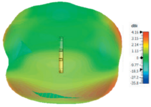
3D Plot Element C Top (2600 MHz)
