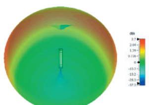
3D Plot Element C Side (1800 MHz)
