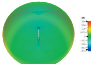
3D Plot Element B Side (1800 MHz)
