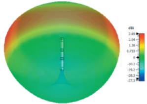
3D Plot Element B Top (1800 MHz)
