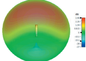
3D Plot Element C Side (750 MHz)
