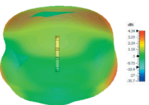
3D Plot Element B Top (2600 MHz)
