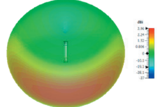
3D Plot Element D Side (750 MHz)
