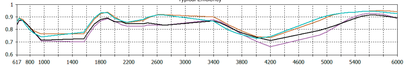
Typical Efficiency*
